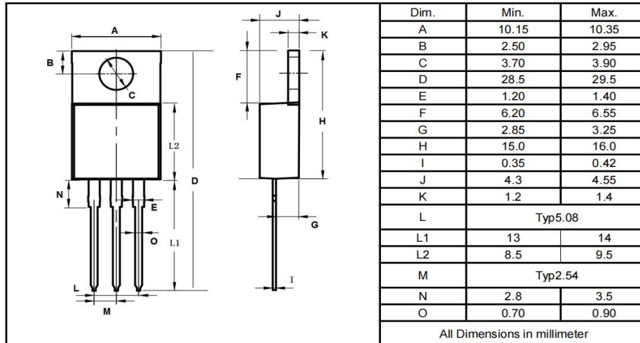
TO-220F
